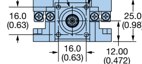
Motor Side End View
