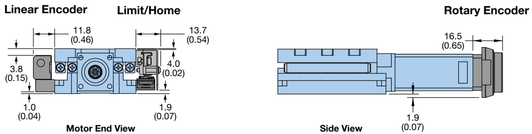
Dimensions – mm (in)
